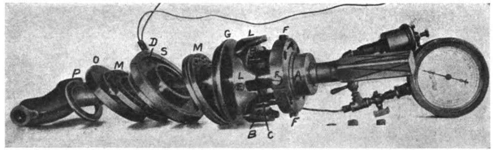
Fig. 3—Transmission dynamometer taken apart to show construction of constituent parts.
